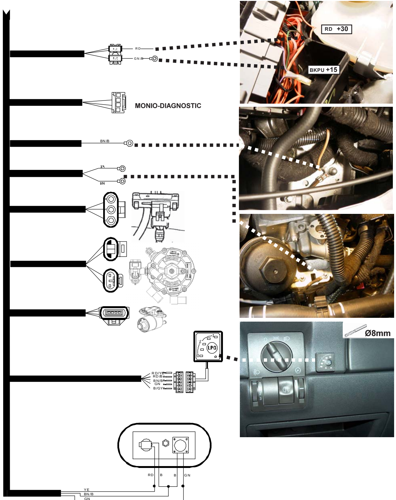
FUSEBOX - bottomsides
