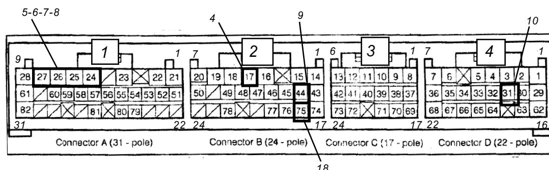
ECU connector
